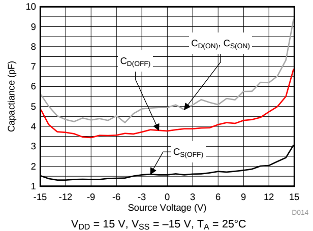
图 14. Capacitance vs Source Voltage
