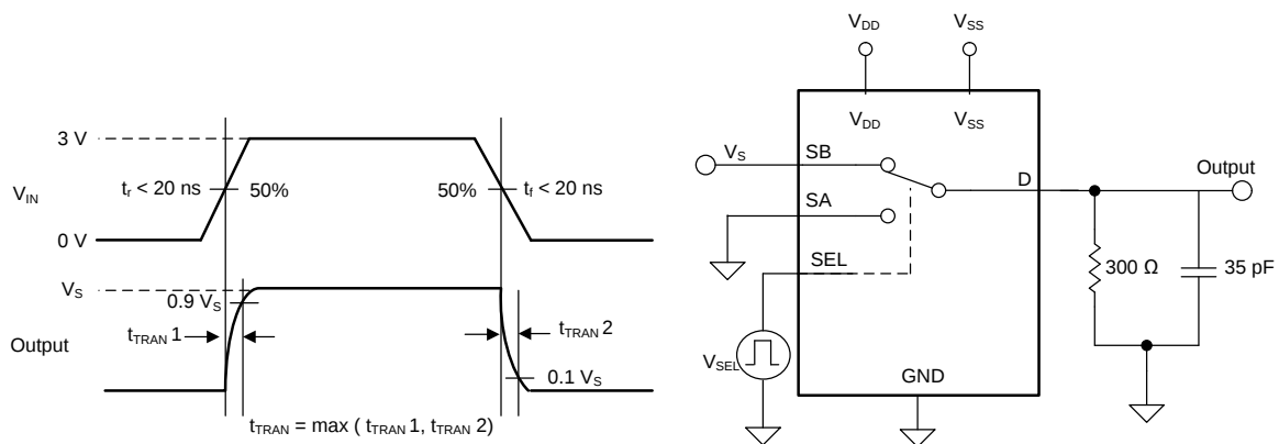
图 20. Transition-Time Measurement Setup
