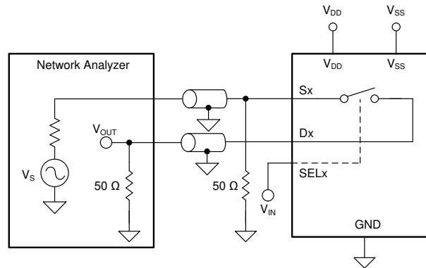
图 23. Off Isolation Measurement Setup
