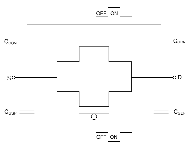
图 28. Transmission Gate Topology
