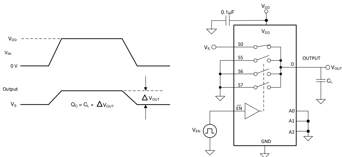
图 8-7. Charge-Injection Measurement Setup
