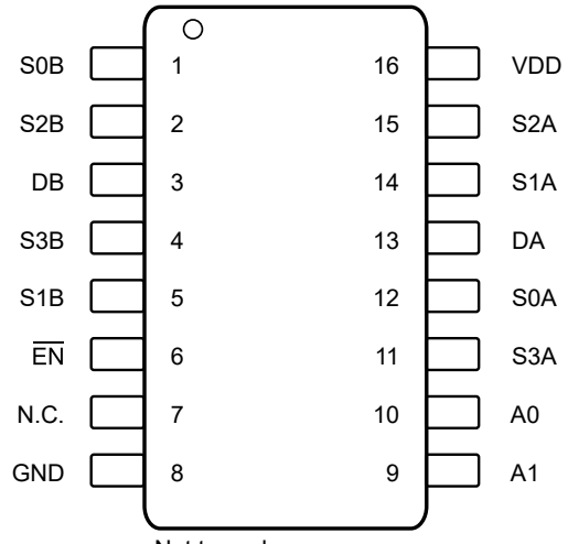
图 6-5. TMUX1309: DYY Package, 16-Pin SOT-23-THIN (Top View)
