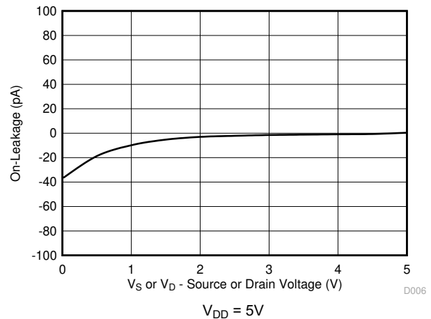
图 5-6. On-Leakage vs Source or Drain Voltage
