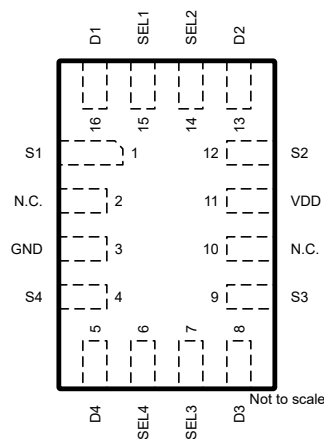
图 5-2. RSV Package, 16-Pin UQFN (Top View)
