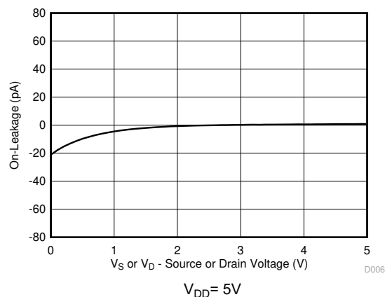
图 9-4. On-Leakage vs Source or Drain Voltage
