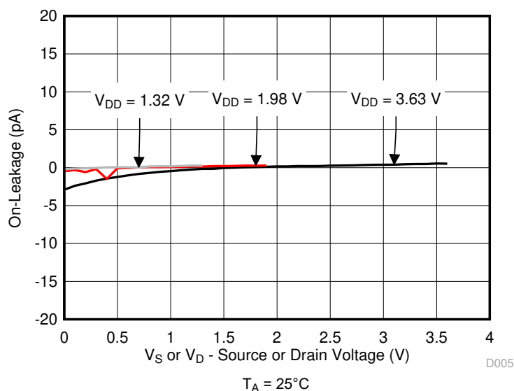
图 9-5. On-Leakage vs Source or Drain Voltage
