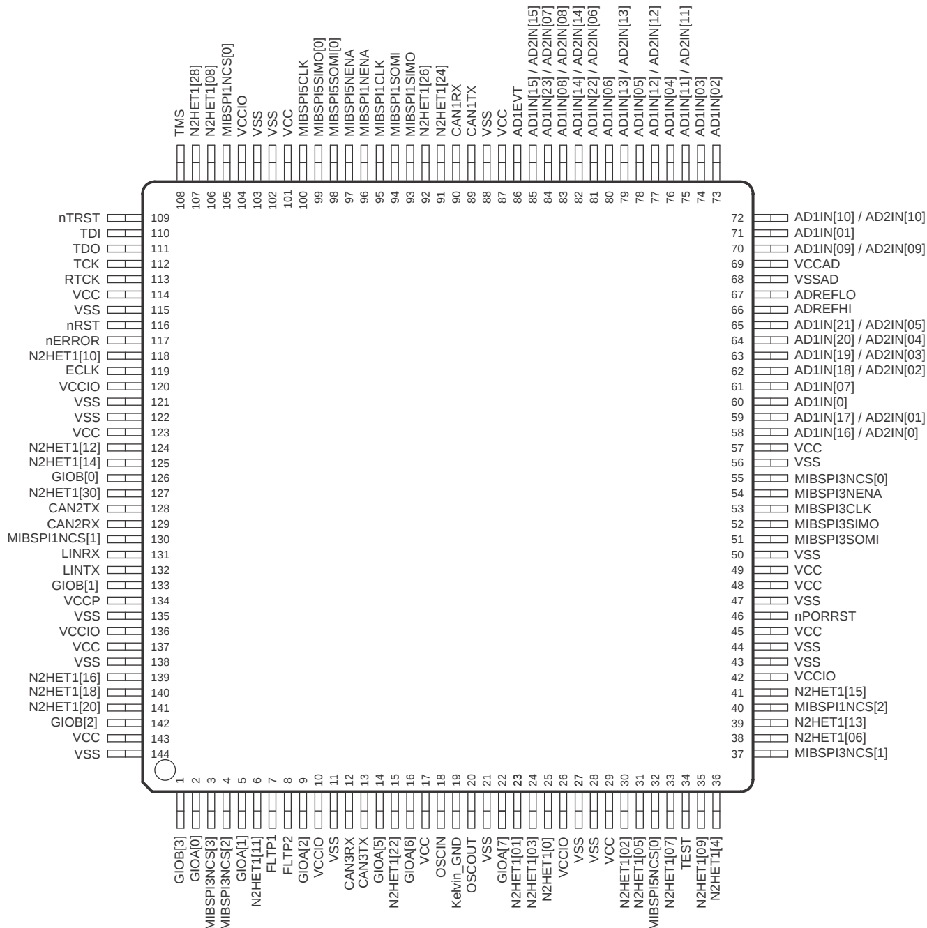
图 3-1. PGE QFP Package Pinout (144-Pin)
