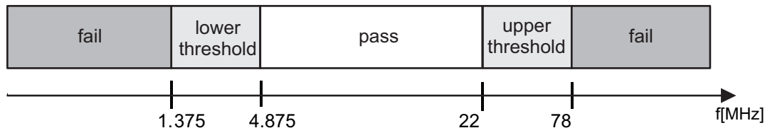
图 5-8. LPO and Clock Detection, Untrimmed HFLPO
