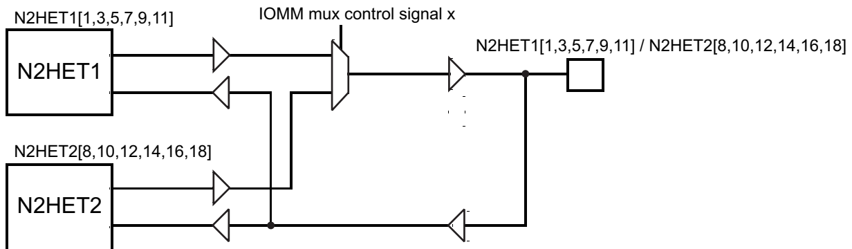
图 6-18. N2HET Monitoring
