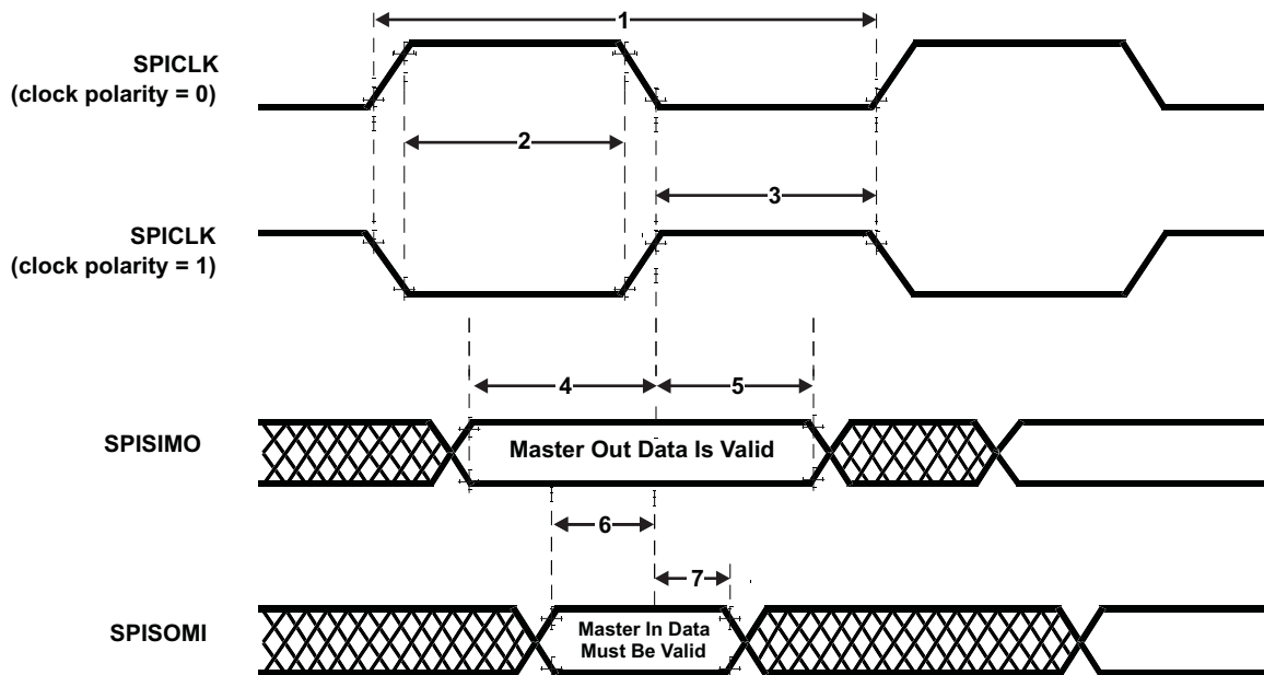
图 6-20. SPI Master Mode External Timing (CLOCK PHASE = 0)
