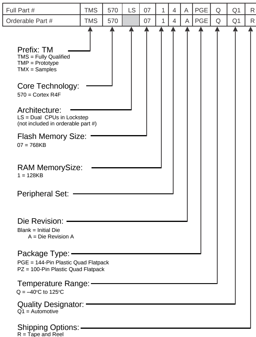
图 8-1. TMS570LS0714-S Device Numbering Conventions
