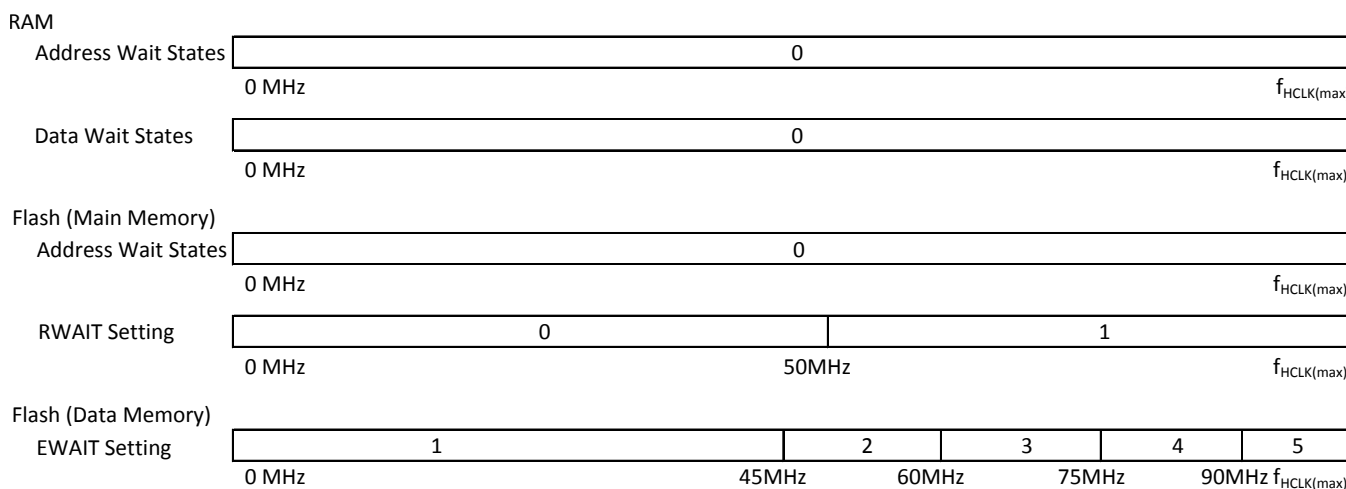
图 4-2. Wait States Scheme — PZ, 100 MHz
