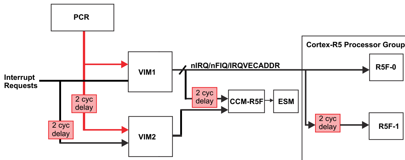
图 7-17. Interrupt Generation
