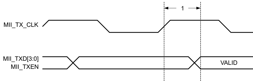
图 8-29. MII Transmit Timing
