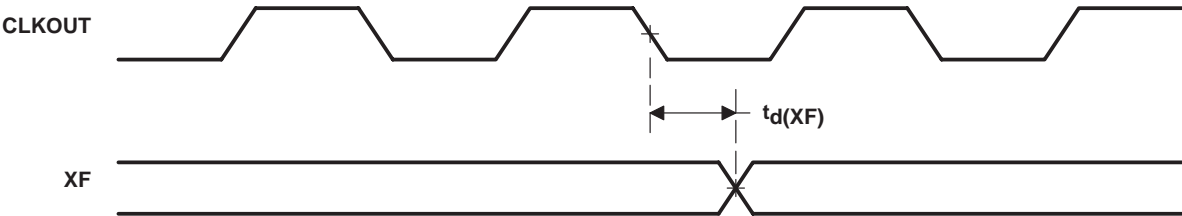
Figure 26. XF Timing
