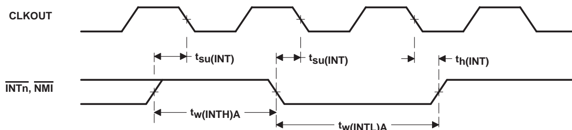
Figure 23. Interrupt Timing
