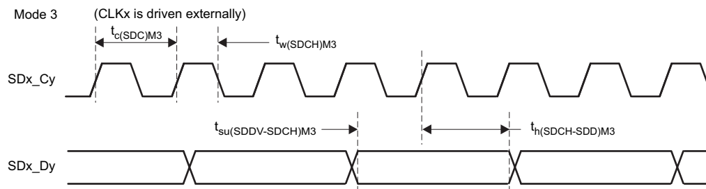
Figure 4-58. SDFM Timing Diagram – Mode 3
