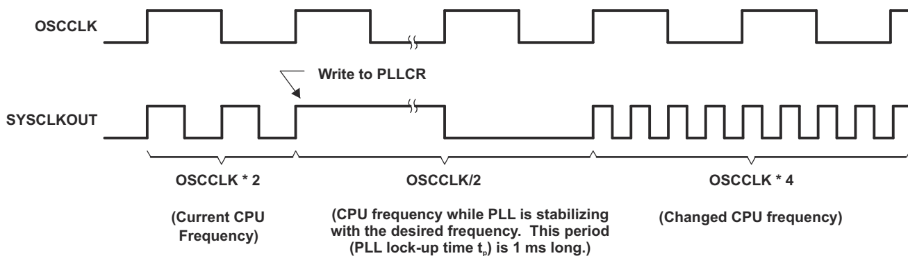
图 7-8. Example of Effect of Writing Into PLLCR Register
