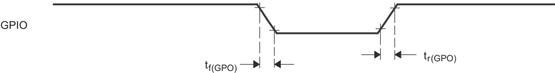
图 8-44. General-Purpose Output Timing
