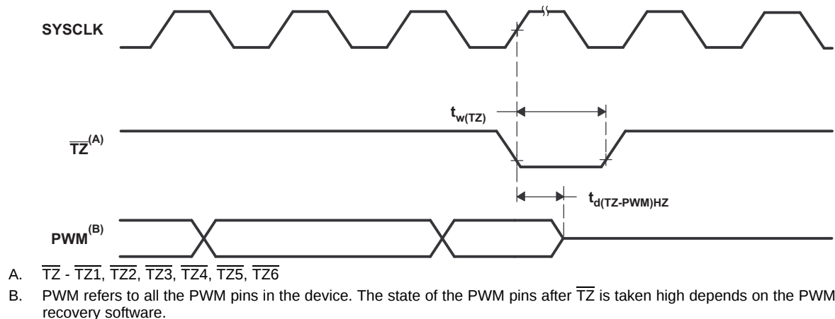
Figure 5-12. PWM Hi-Z Characteristics
