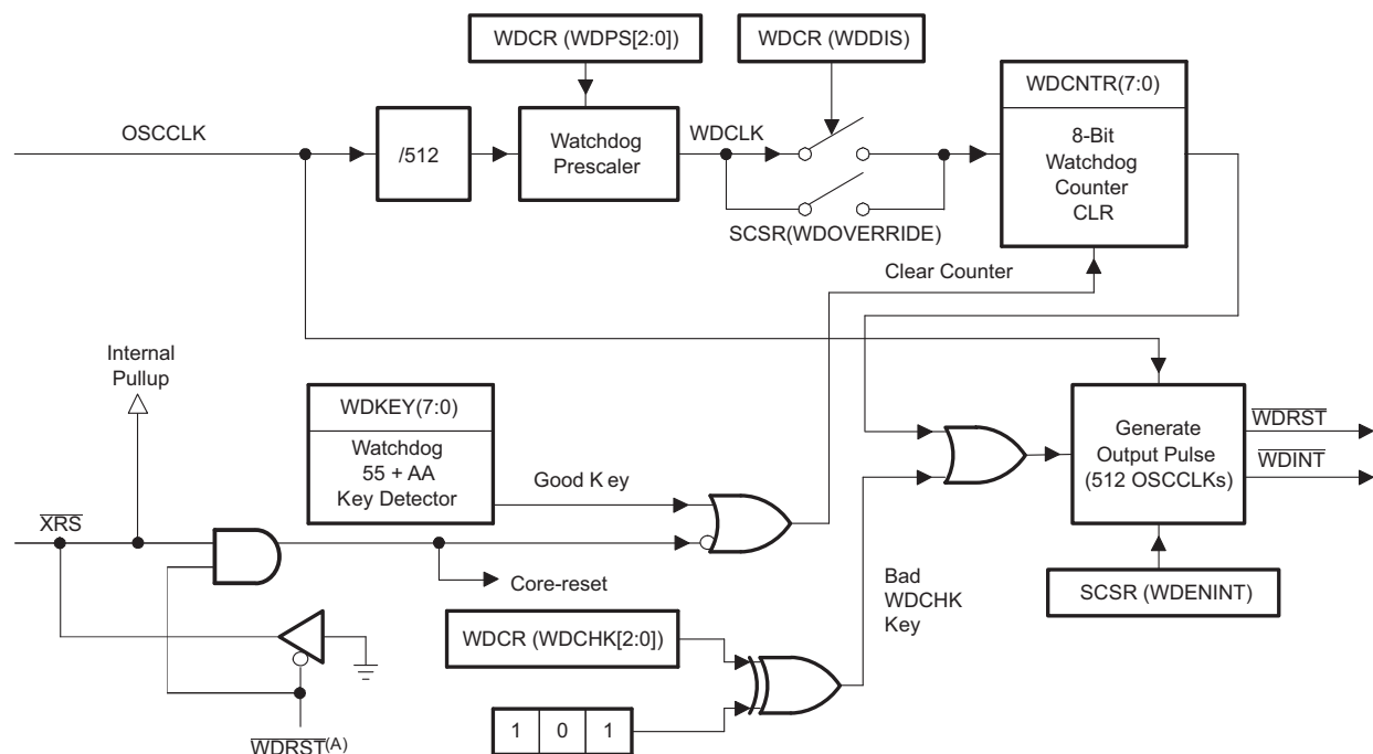
Figure 6-21. Watchdog Module
