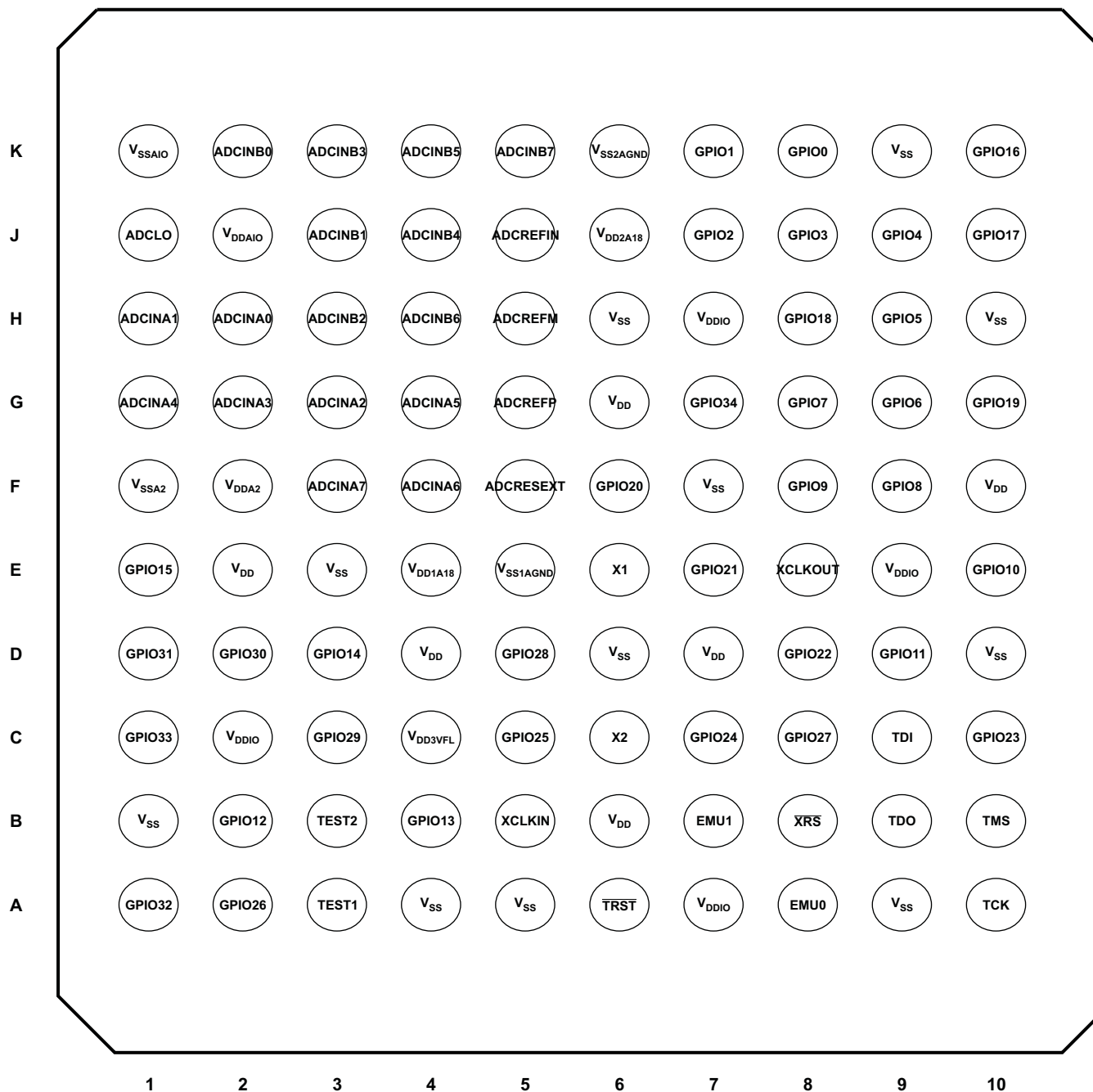
BOTTOM VIEW
