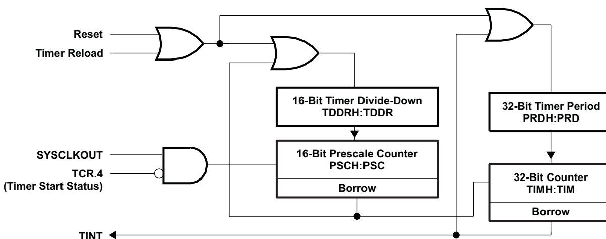
Figure 6-1. CPU-Timers
