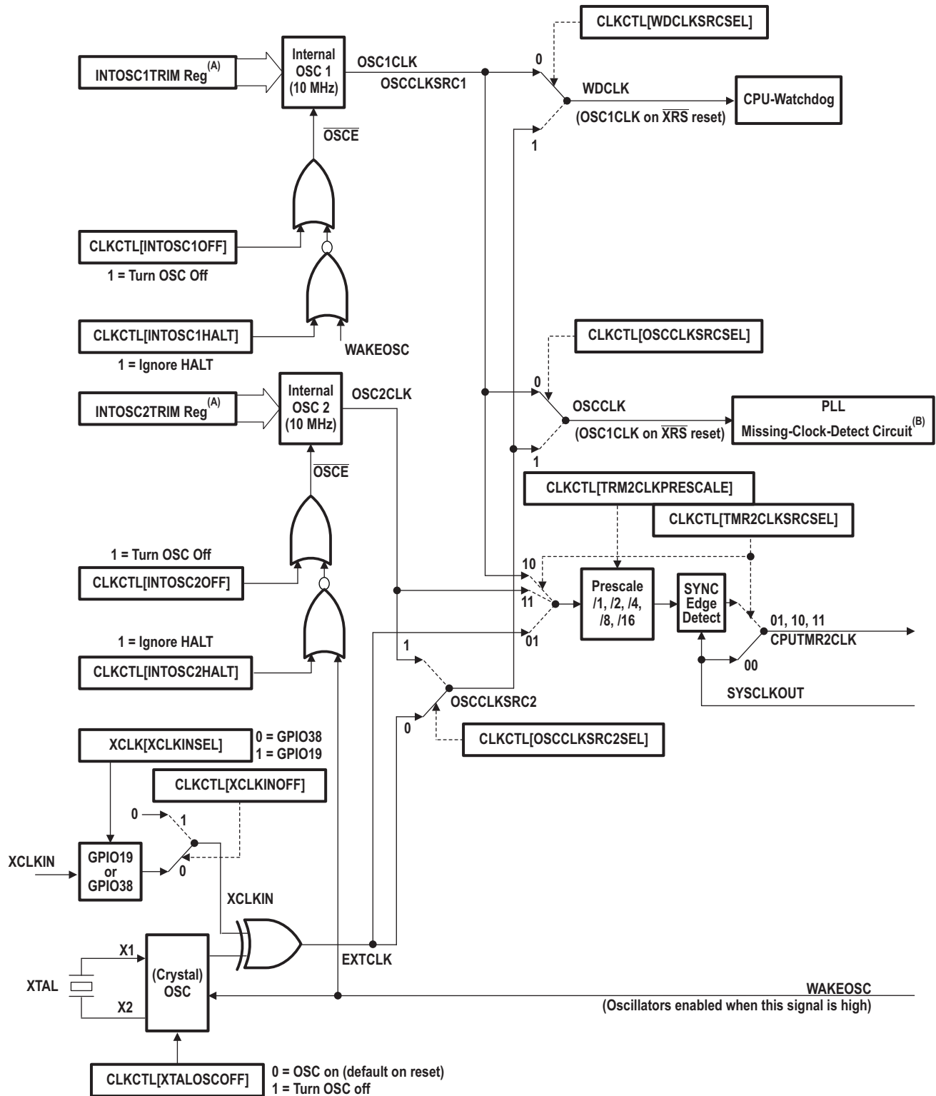
Figure 2-6. Clock Tree
