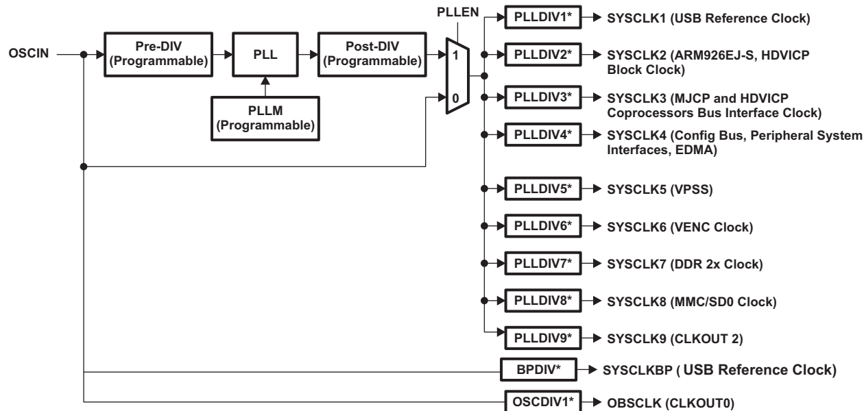
Figure 4-3. PLLC1 Configuration
