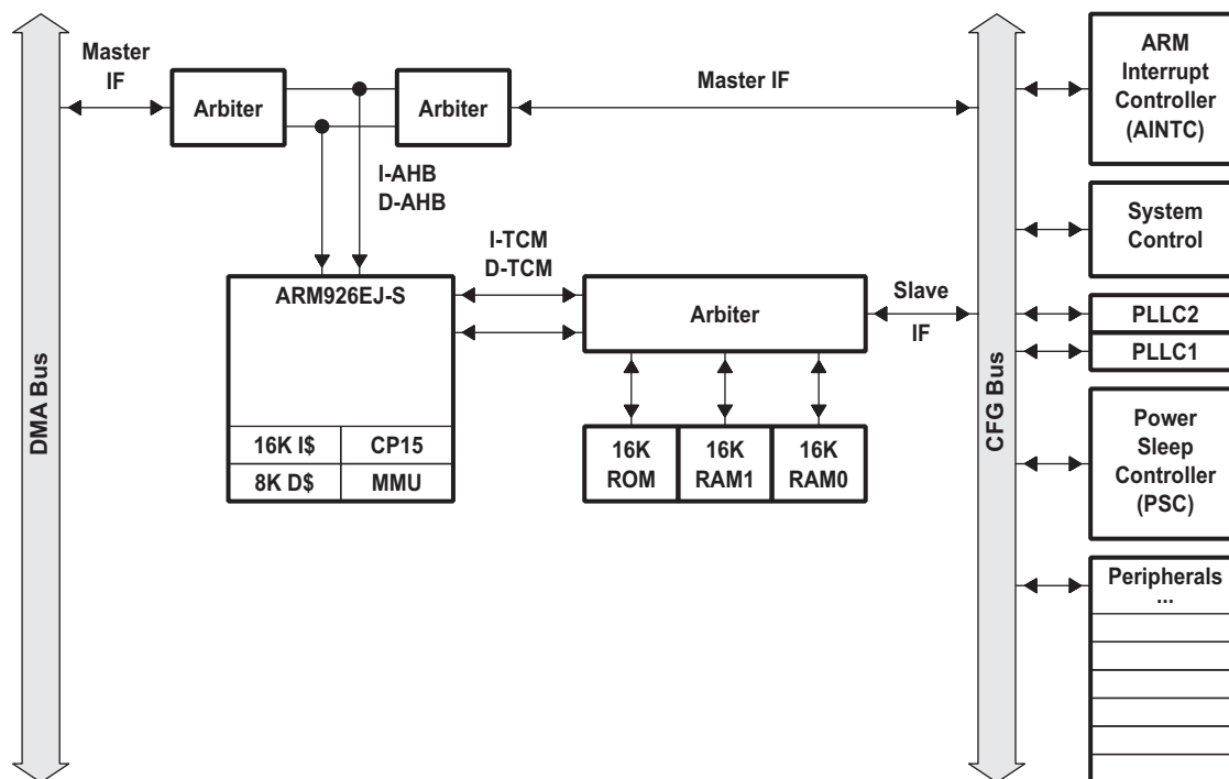
Figure 3-1. ARM Subsystem Block Diagram
