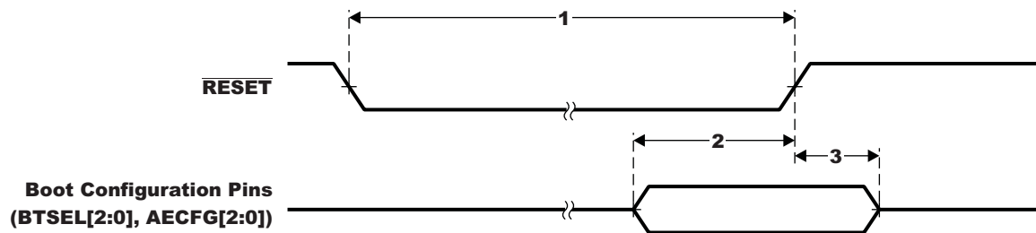
Figure 7-4. Reset Timing
