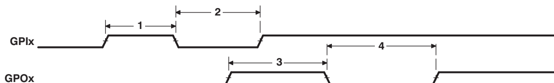
Figure 7-11. GPIO Port Timing
