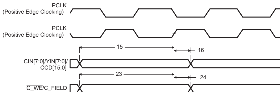
Figure 7-33. VPFE (ISIF) Master Mode Input Data Timing
