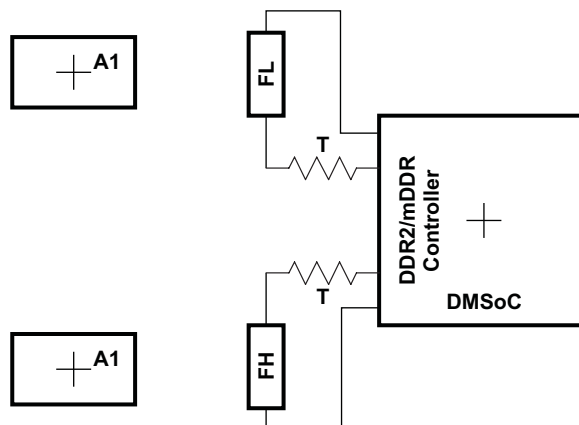
Figure 7-26. DQGATE Routing
