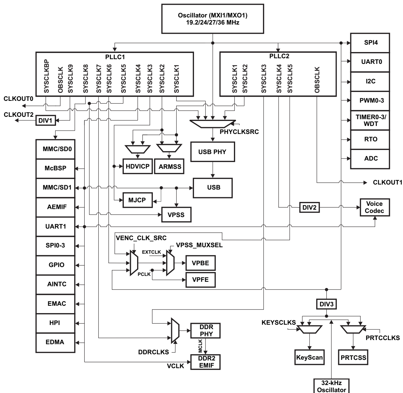
Figure 4-2. Clocking Architecture
