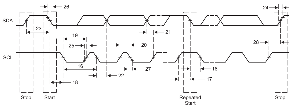
Figure 7-33 I 2 C Transmit Timings
