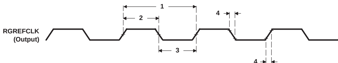
Figure 7-68. RREFCLK Timing
