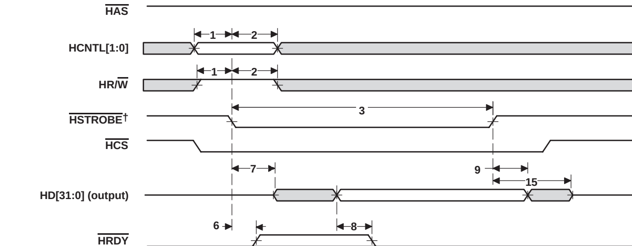
Figure 7-36. HPI32 Read Timing ( \overline{\text{HAS}} Not Used, Tied High)
