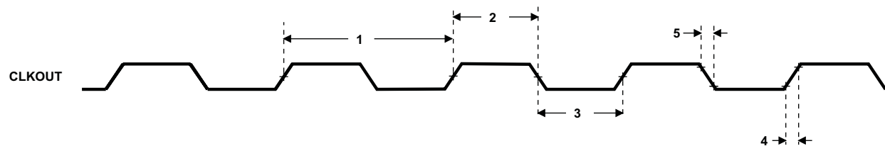
Figure 5-10. CLKOUT Timing
