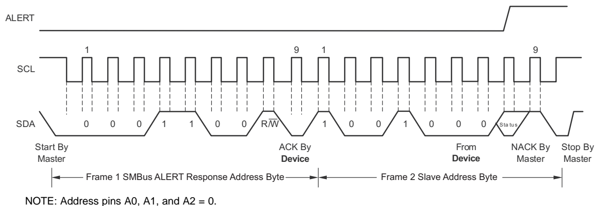
Figure 10. Timing Diagram for SMBus ALERT
