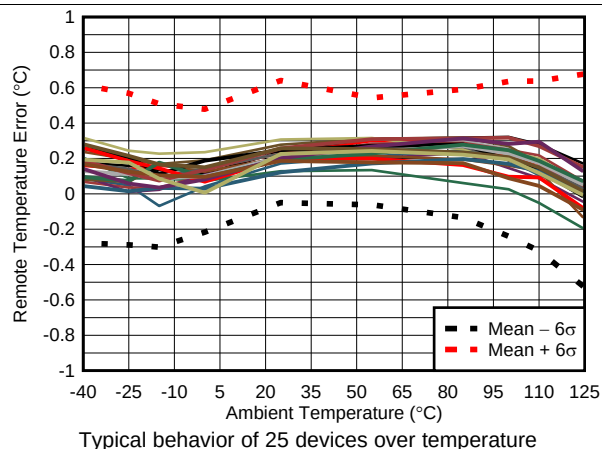
Figure 3. Remote Temperature Error vs Ambient Temperature
