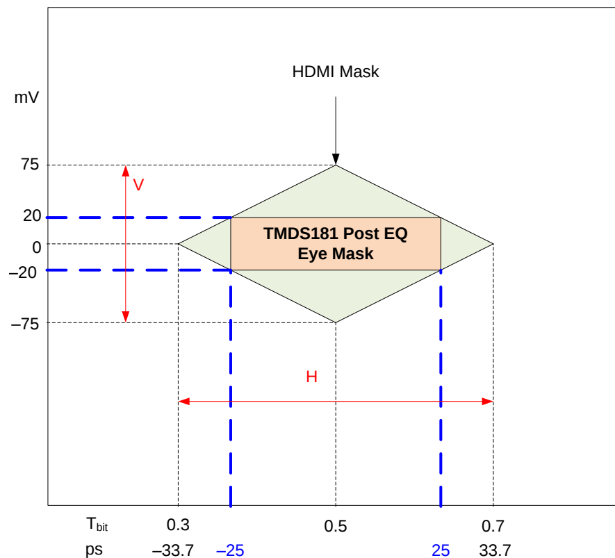
Figure 12. HDMI Output Jitter Measurement
