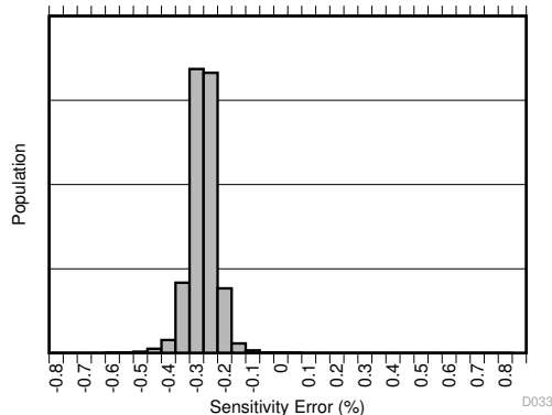
TMCS1101AxU
