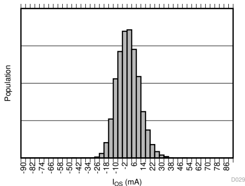
TMCS1101A1B
