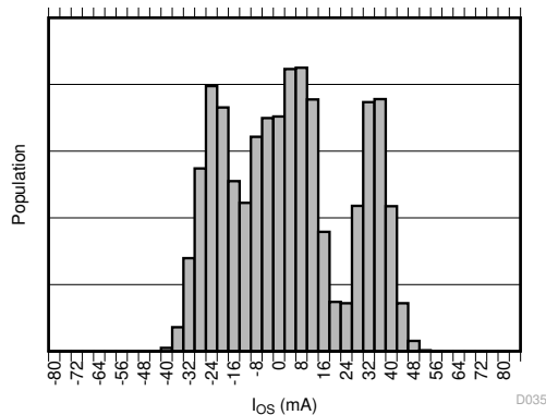
TMCS1101A2U
