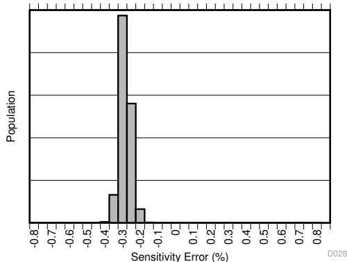
TMCS1101AxB
