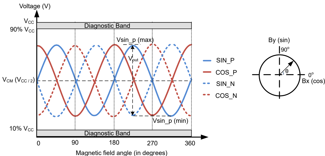
图 6-4. AMR Sensor Outputs Magnetic Response
