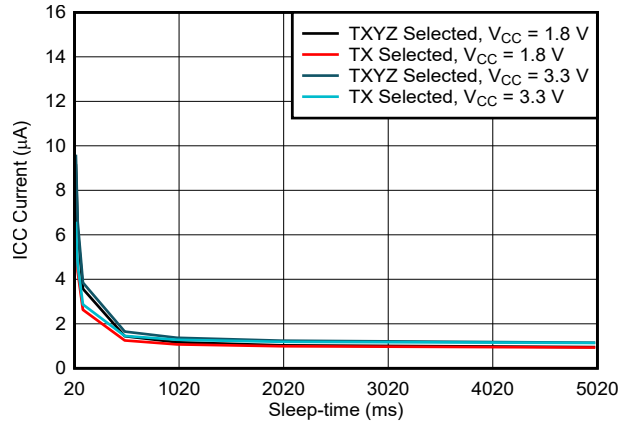
图 6-4. Average ICC vs W&S Mode Sleep Time
