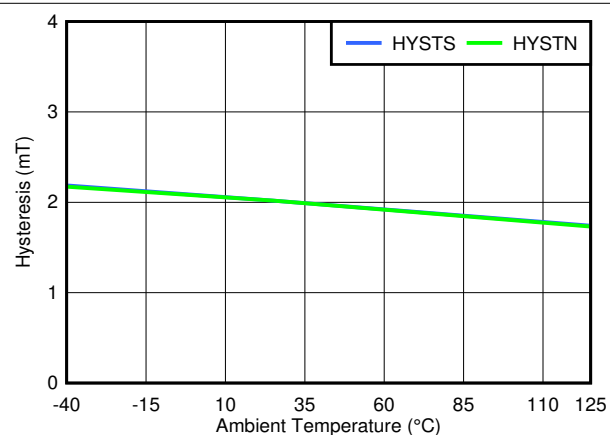
图 7-5. TMAG5123B Hysteresis vs Temperature
