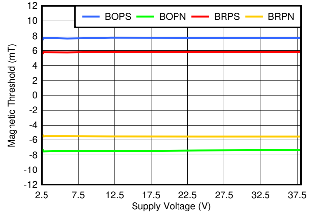
图 7-8. TMAG5123C Magnetic Thresholds vs Voltage
