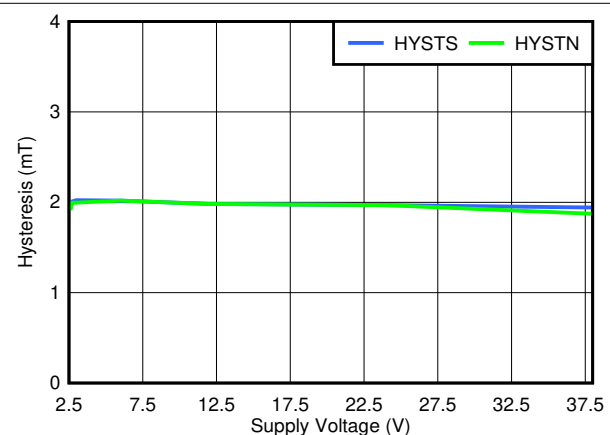
图 7-6. TMAG5123B Hysteresis vs Supply Voltage
