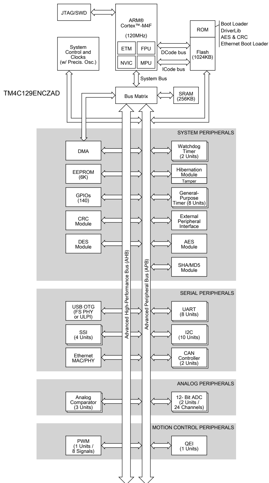
Figure 1-1. Tiva™ TM4C129ENCZAD Microcontroller High-Level Block Diagram
