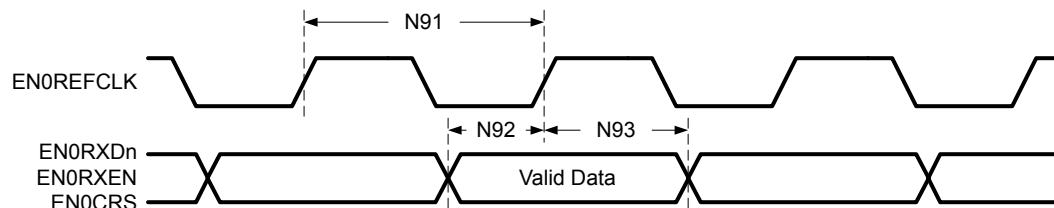
Figure 30-43. RMII Receive Timing
