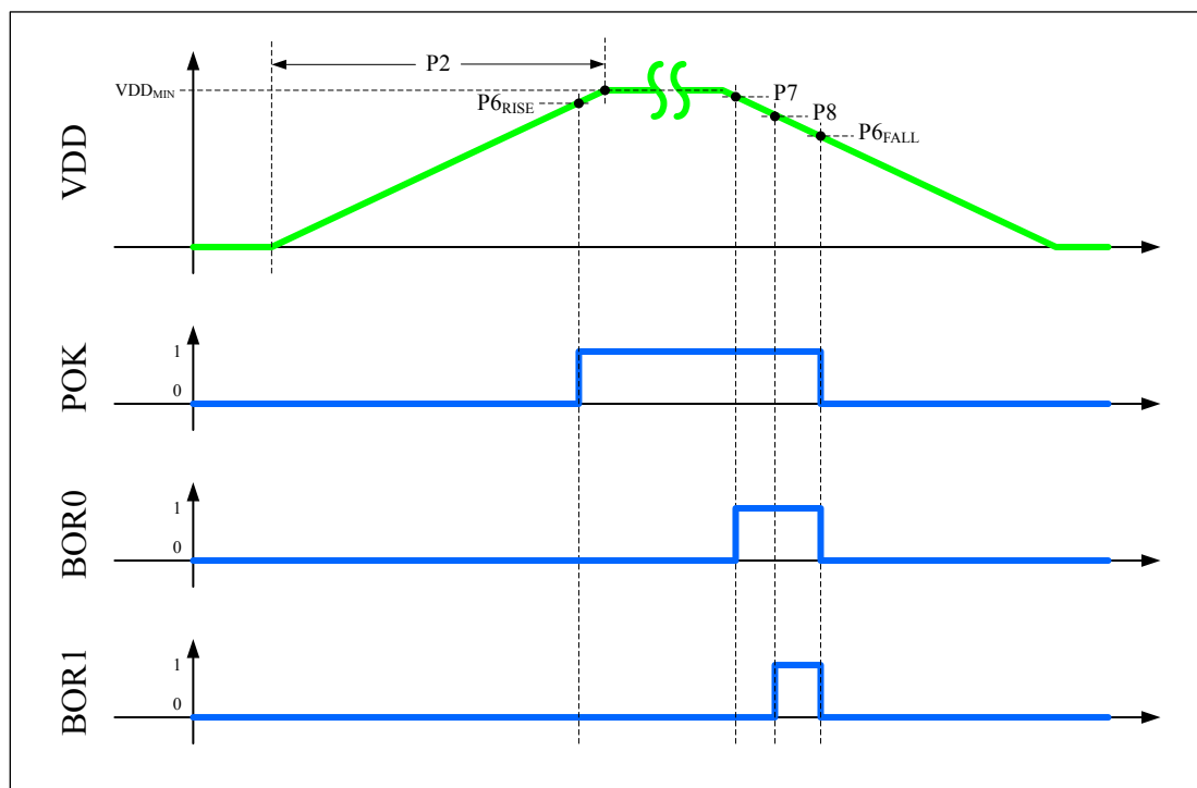
图 22-5. Power and Brown-Out Assertions versus V_{DD} Levels
