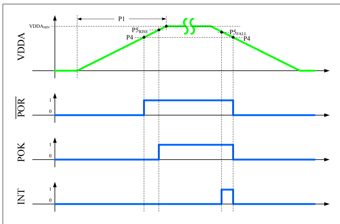
图 21-4. Power Assertions versus VDDA Levels
