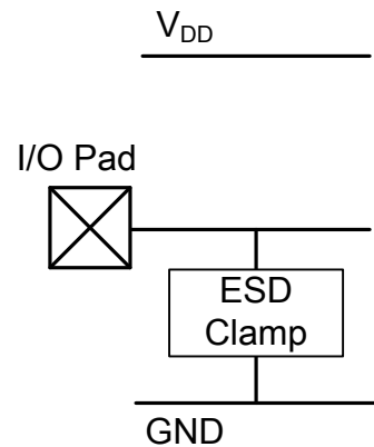
图 21-16. ESD Protection on Fail-Safe Pins
