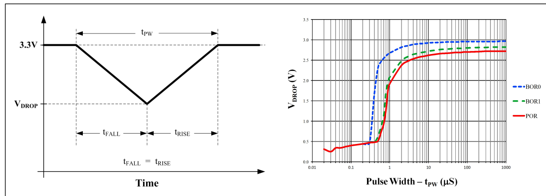
图 20-7. POR-BOR0-BOR1 VDD Glitch Response
