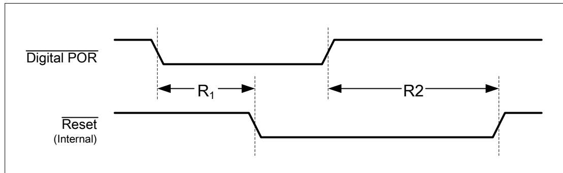
图 20-9. Digital Power-On Reset Timing
