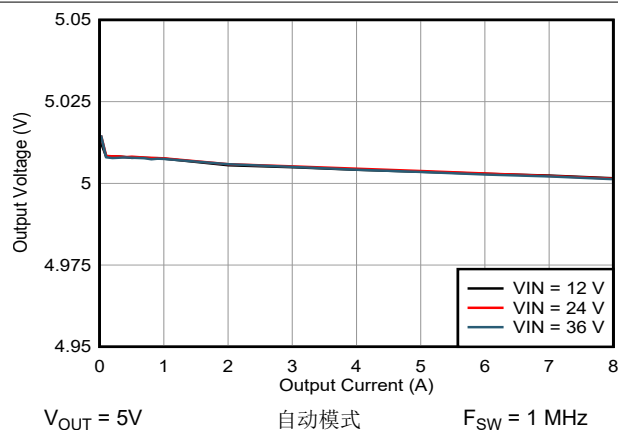
图 9-5. V_{OUT} = 5V 时的负载调节
