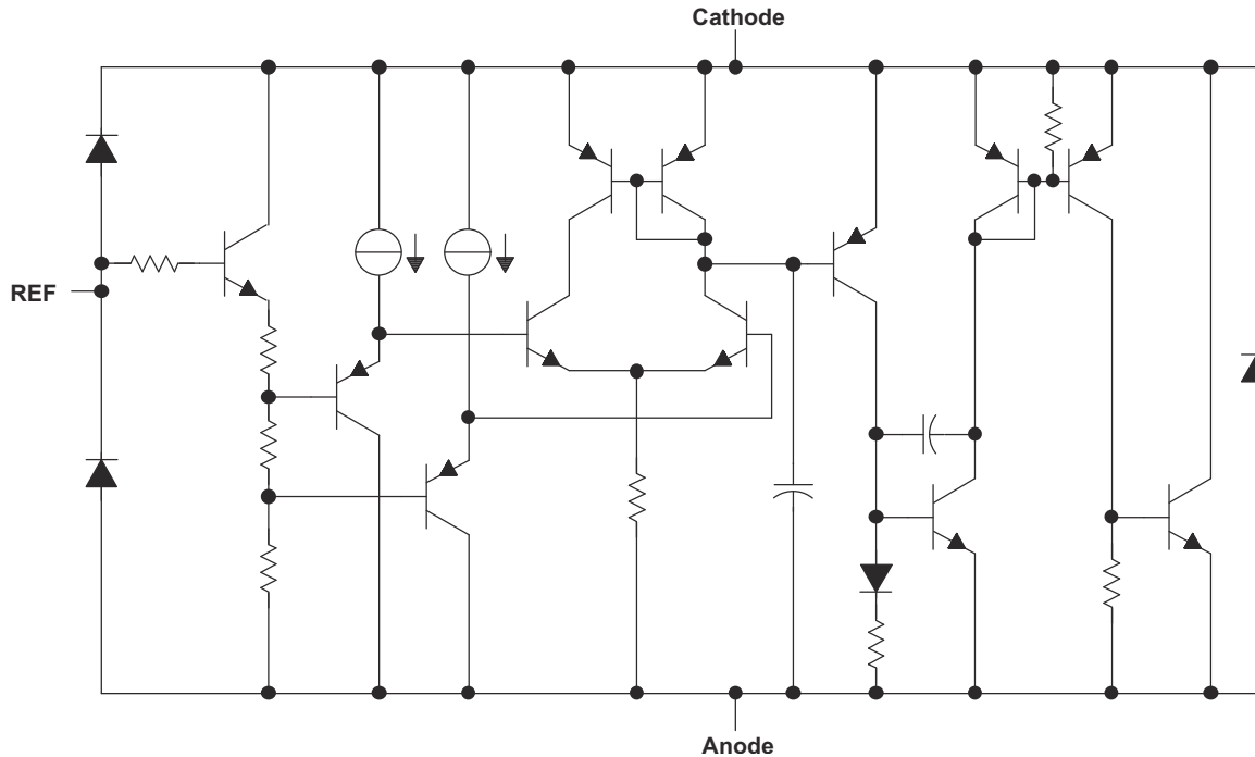
图 7-2. Detailed Schematic
