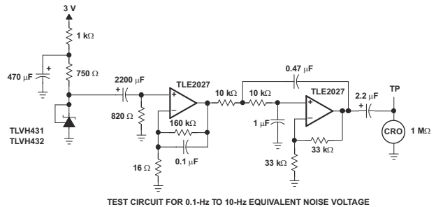
图 5-10. Equivalent Input Noise Voltage
