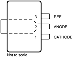
图 4-7. TLVH432 PK Package 3-Pin SOT-89 Top View
