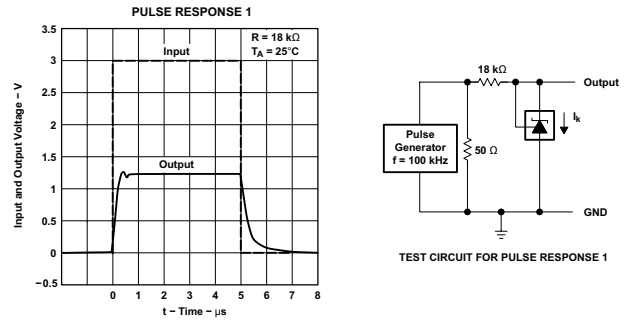
图 5-12. Pulse Response 1
