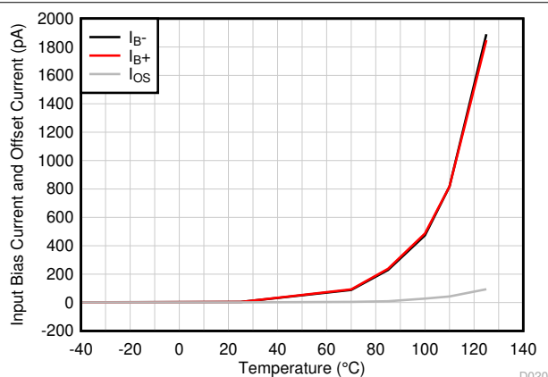
图 5-10. Input Bias Current and Offset Current vs Temperature
