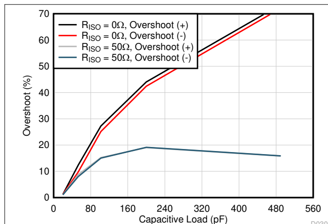
图 6-3. Small-Signal Overshoot vs Capacitive Load (20mV pp Output Step, G = +1)
