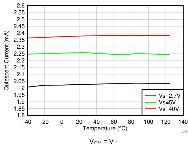
图 5-23. Quiescent Current vs Temperature
