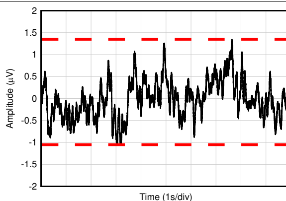
图 5-20. 0.1Hz to 10-Hz Noise
