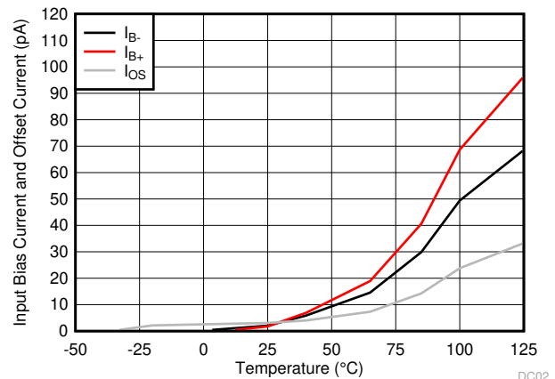
图 5-6. Input Bias Current vs Temperature
