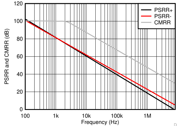
图 5-10. CMRR and PSRR vs Frequency (Referred to Input)
