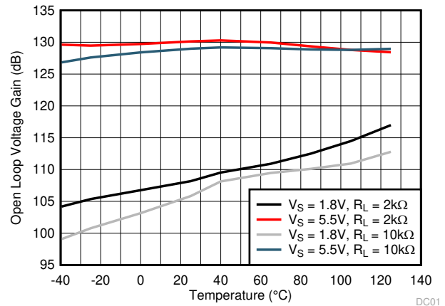
图 5-14. Open Loop Voltage Gain vs Temperature
