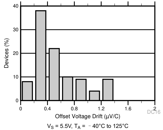
图 5-2. Offset Voltage Drift Distribution
