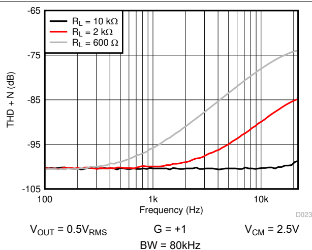
图 6-29. THD + N vs Frequency
