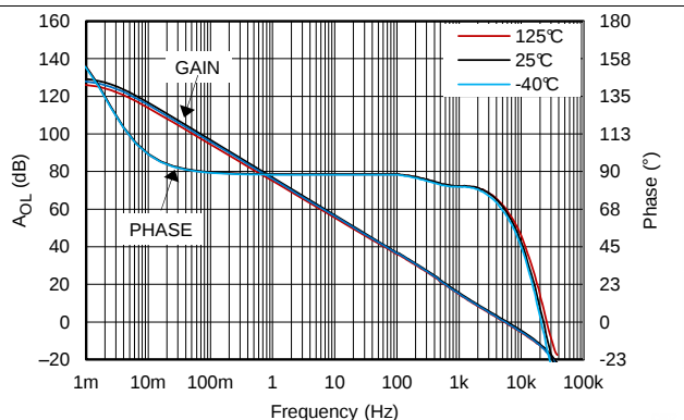
Figure 26. 开环增益和相位, 3.3V, 10MΩ 负载
