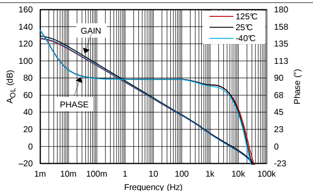
Figure 25. 开环增益和相位, 5V, 10MΩ 负载
