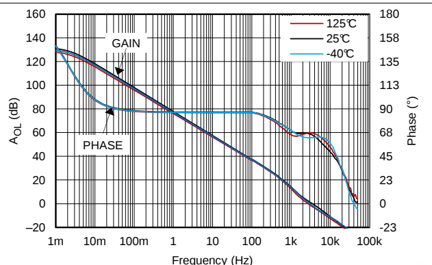
Figure 27. 开环增益和相位, 5V, 1MΩ 负载
