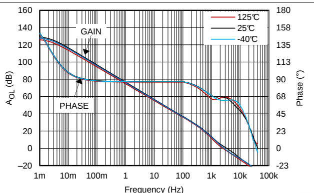
Figure 28. 开环增益和相位, 3.3V, 1MΩ 负载
