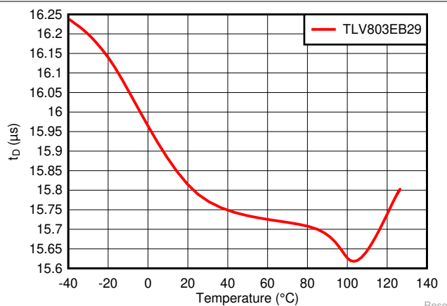
图 7-22. Reset Delay Time Verses Temperature for TLV803EB29
