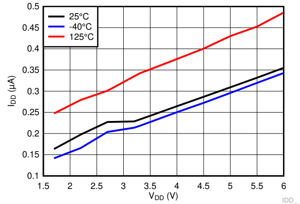
图 7-4. Supply Current Versus Supply Voltage for TLV809EA29
