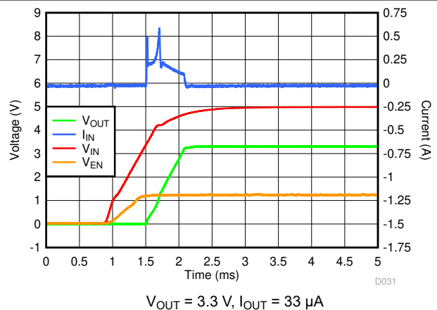
图 6-24. Startup Inrush Current With C_{OUT} = 47\text{ }\mu\text{F}
