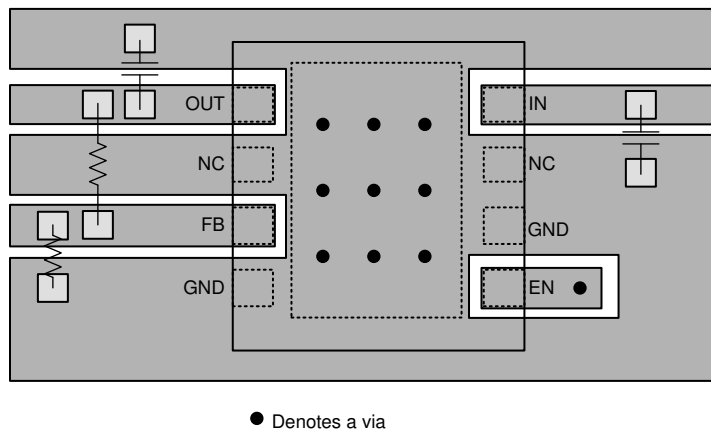
图 8-5. Layout Example for the Adjustable Version
