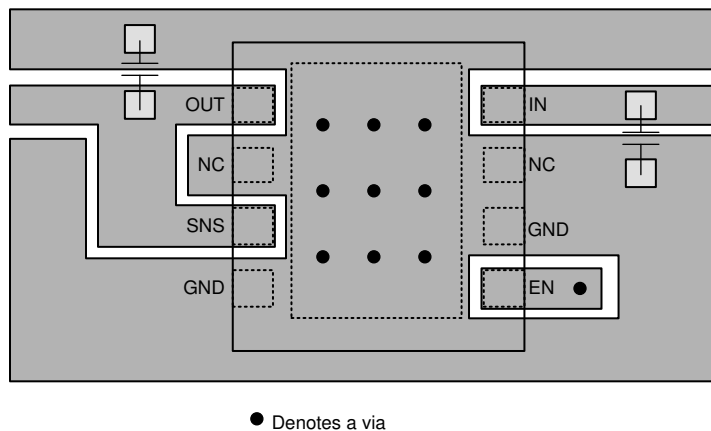
图 8-6. Layout Example for the Fixed Version
