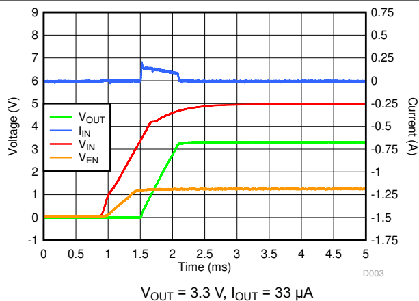
图 6-23. Startup Inrush Current With C_{OUT} = 22\text{ }\mu\text{F}
