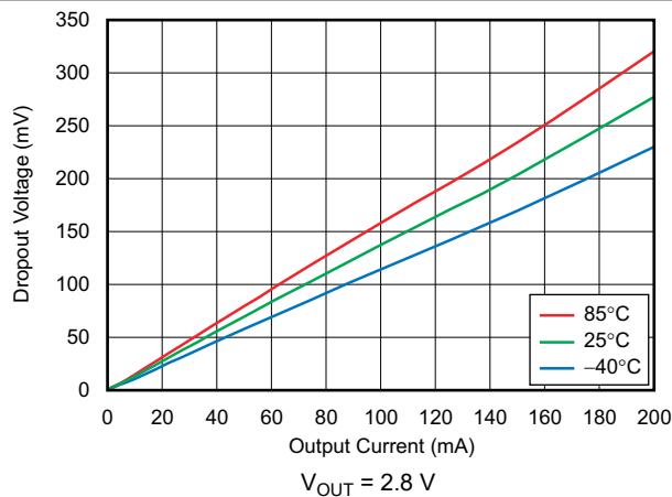
图 6-15. Dropout Voltage vs Output Current
