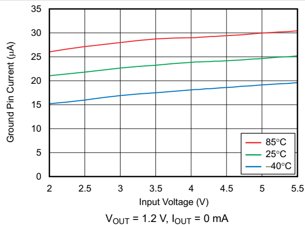
图 6-17. Ground Pin Current vs Input Voltage
