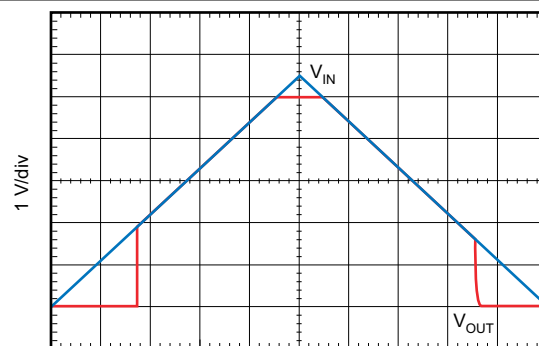
图 6-56. V_{IN} Ramp Up, Ramp Down Response
