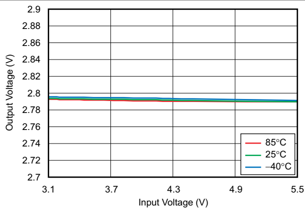
图 6-8. Line Regulation
