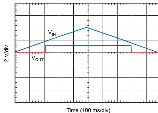
图 8-9. V_{IN} Ramp Up, Ramp Down Response
