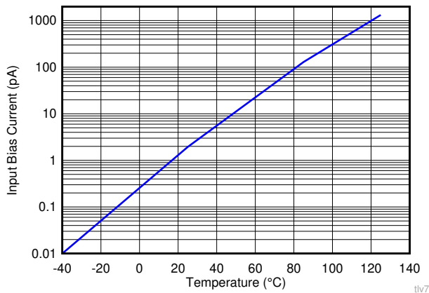
A. V_{CC} = 5\text{V} 图 5-17. Input Bias Current vs Temperature
