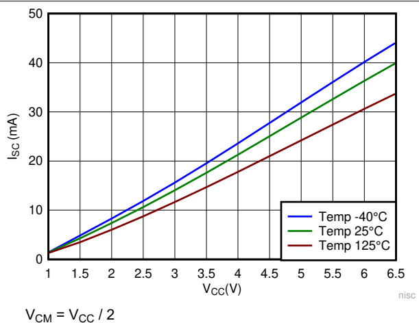
图 6-20. Output Short Circuit (Sink) vs V_{CC}
