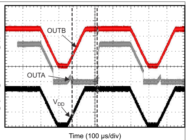
图 9-6. Start-Up Delay (OUT Pulled Up to V_{DD} )
