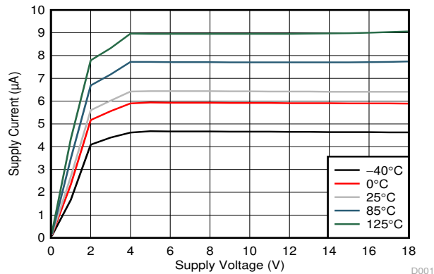
图 7-2. Supply Current ( I_{DD} ) vs Supply Voltage ( V_{DD} )
