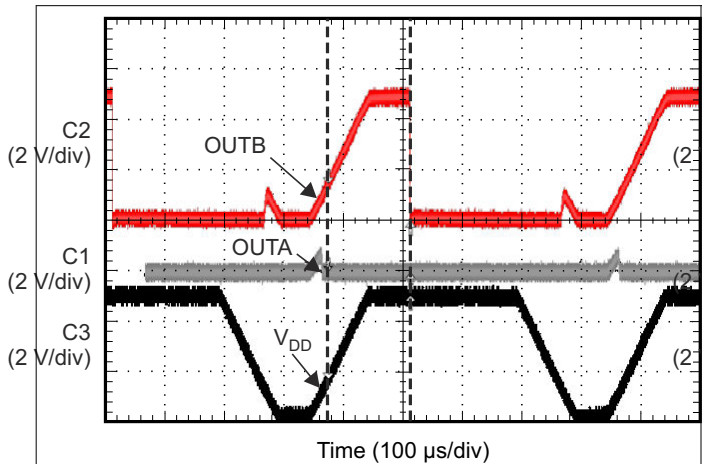
图 9-5. Start-Up Delay (OUT Pulled Up to V_{DD} )
