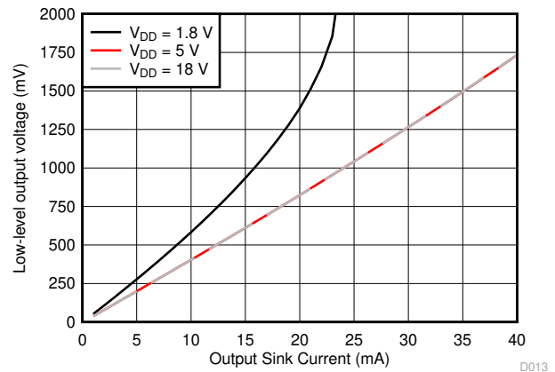
图 7-13. Output Voltage Low ( V_{OL} ) vs Output Sink Current (125°C)
