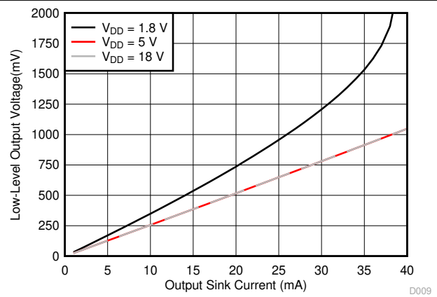
图 7-9. Output Voltage Low ( V_{OL} ) vs Output Sink Current (-40°C)
