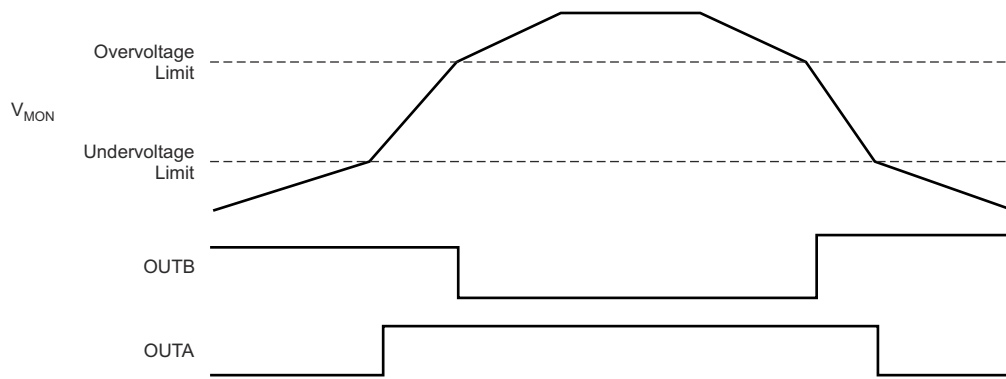
图 8-2. Window Comparator Timing Diagram
