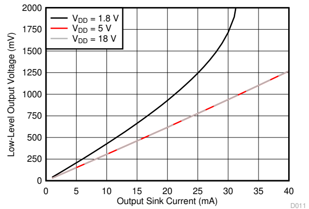
图 7-11. Output Voltage Low ( V_{OL} ) vs Output Sink Current (25°C)
