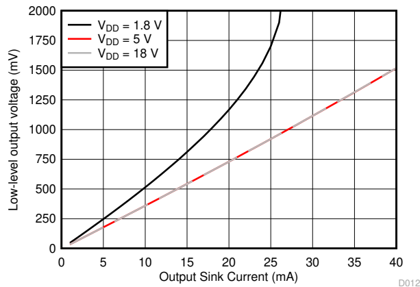
图 7-12. Output Voltage Low ( V_{OL} ) vs Output Sink Current (85°C)
