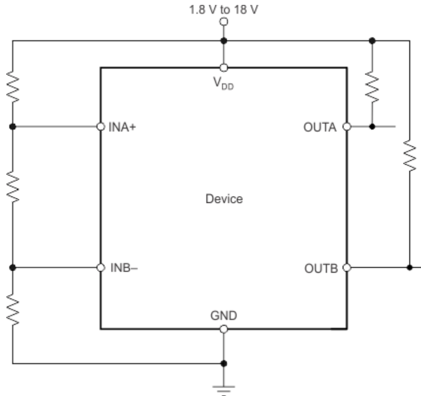
图 9-2. Monitoring the Same Voltage as V_{DD}
