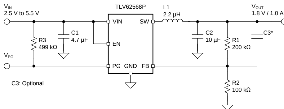
图 5. TLV62568 1.8-V Output Application
