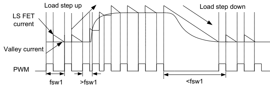
图 10. Operation in Load Transient
