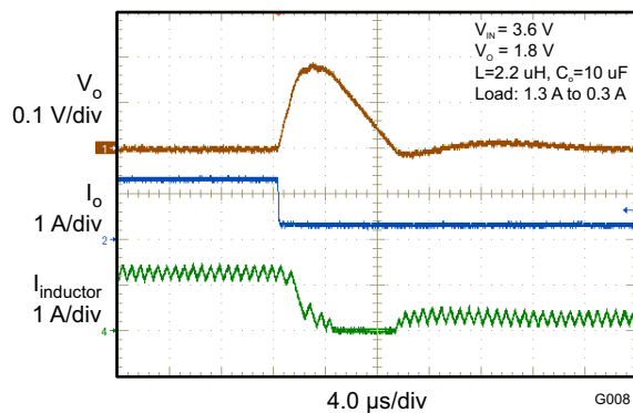
图 18. Typical Application (PFM Mode)
